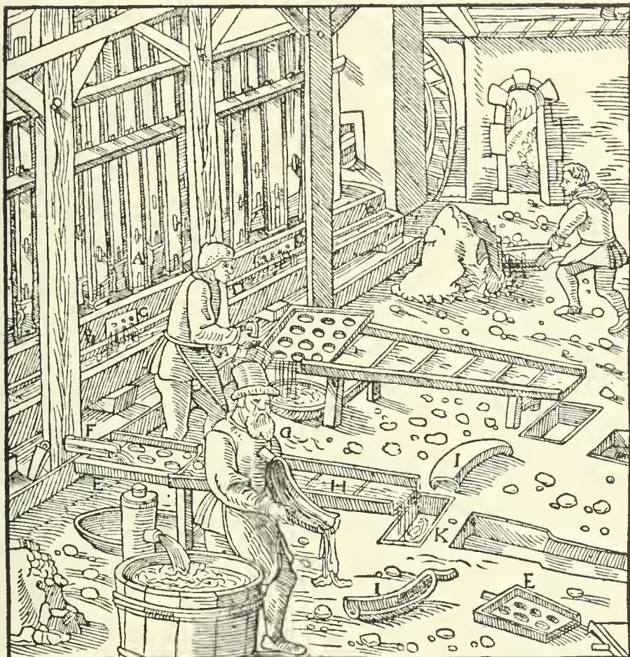
A—STAMPS. B—MORTAR. C—PLATES FULL OF HOLES. D—TRANSVERSE LAUNDER. E—PLANKS FULL OF CUP-LIKE DEPRESSIONS. F—SPOUT. G—BOWL INTO WHICH THE CONCENTRATES FALL. H—CANVAS STRAKE. I—BOWLS SHAPED LIKE A SMALL BOAT. K—SETTLING-PIT UNDER THE CANVAS STRAKE.
